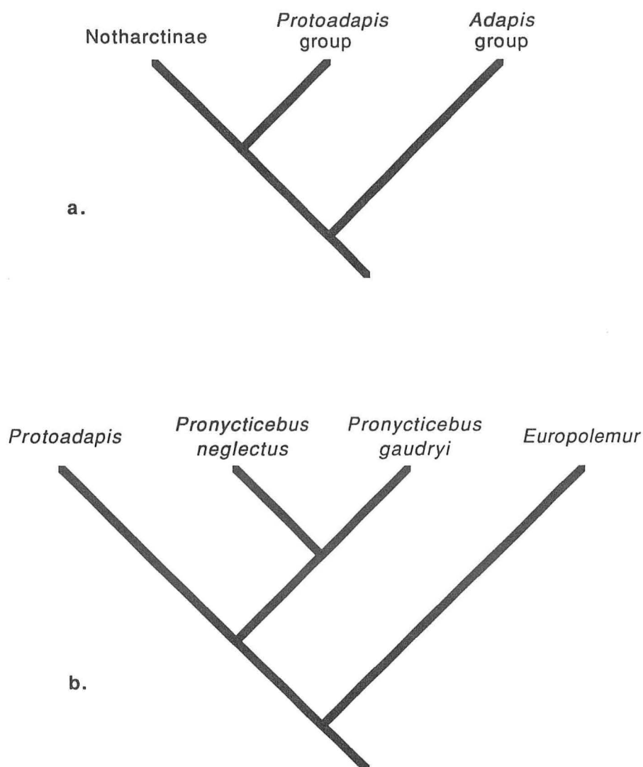
Figure 3: Phylogenetic hypotheses. Suggested relationships for a: higher North American and European adapid taxa of the Eocene, and for b: Pronycticebus neglectus .
